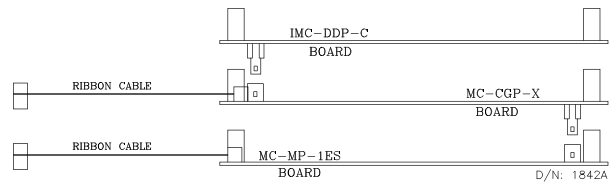
FIGURE A.4 Computer Swing Panel Boards Unsnapped
