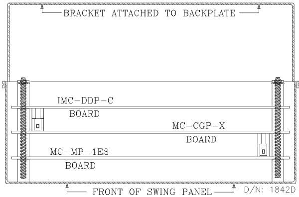
FIGURE A.3 Computer Swing Panel Boards Snapped Together
