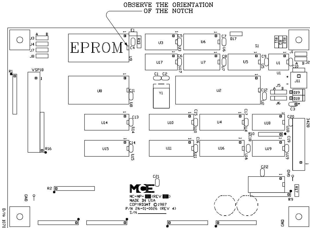
FIGURE A.5 EPROM Location on the Main Processor Board (MC-MP-1ES)
